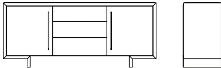
80" W X 20" D X 34" H LAYOUT A
