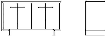
60" W X 20" D X 34" H LAYOUT B
