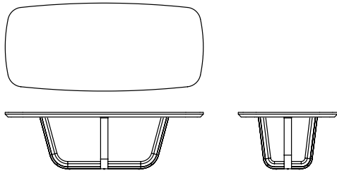
108" W X 48" D X 29" H FUSED BASE
